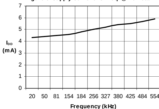
Figure 5: Supply Current vs Freq. @ No Load
