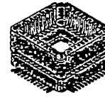
42-PIN CERAMIC MODULE (MDP-42C-P04)
