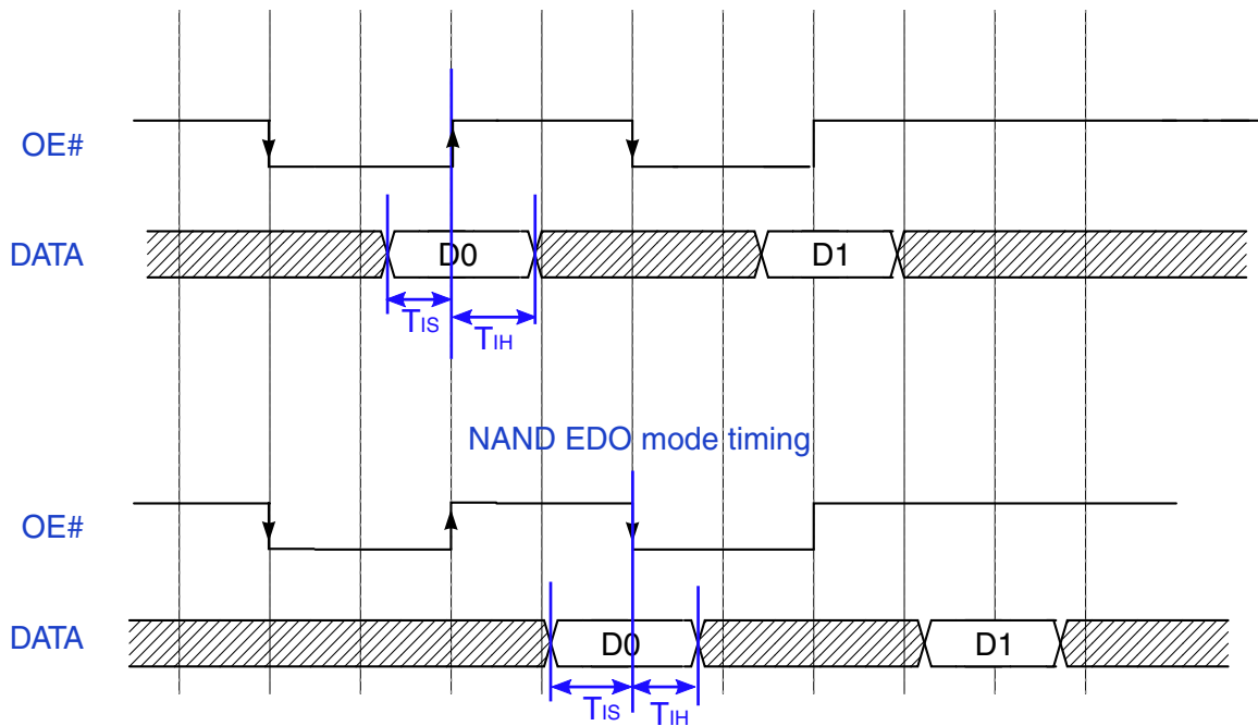
NAND non-EDO mode and NOR/PSRAM/8080 timing
