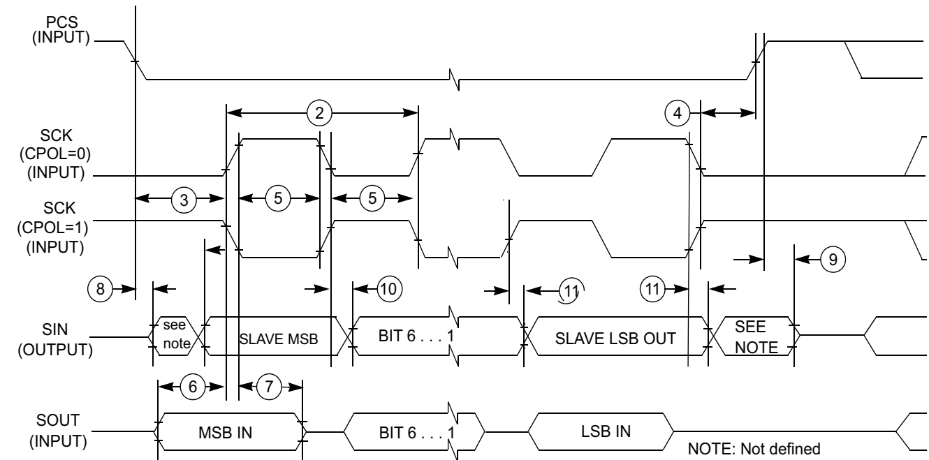
Figure 41. LPSPI Slave mode timing (CPHA = 0)
