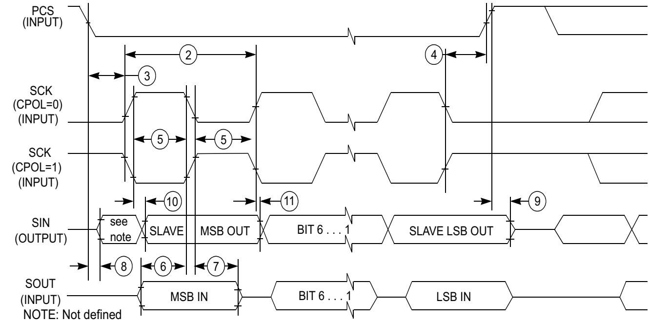
Figure 42. LPSPI Slave mode timing (CPHA = 1)
