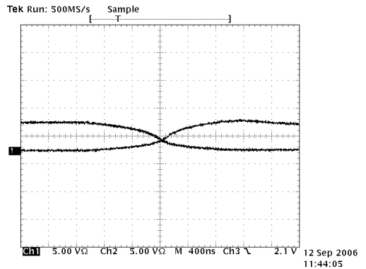
Driver output Waveform High to Low (SP3080-SP3082)
