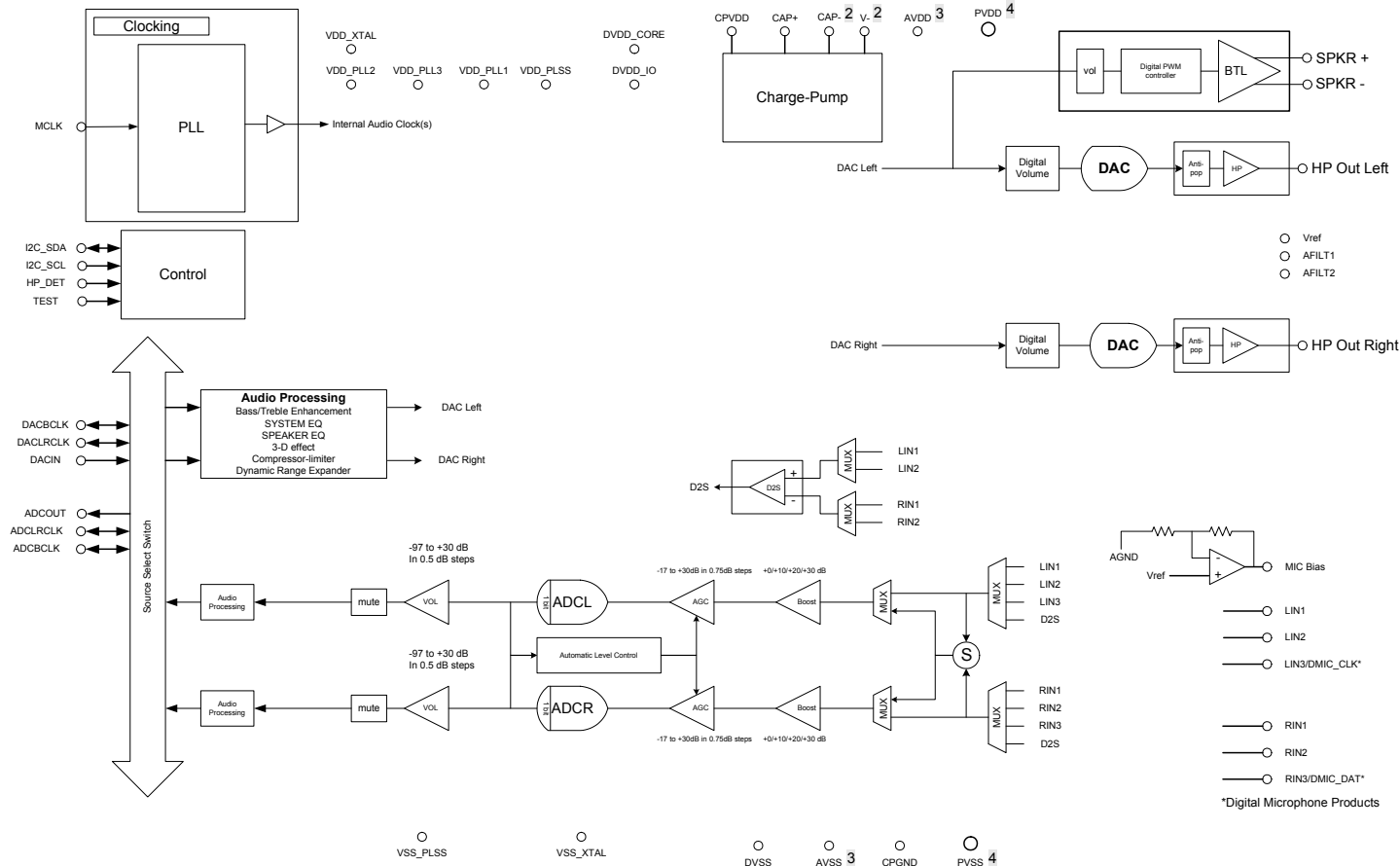
Figure 1. Block Diagram
