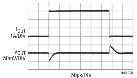
1.2V Transient Response
