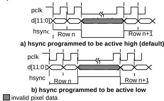
Figure 37. hsync in Level Mode
