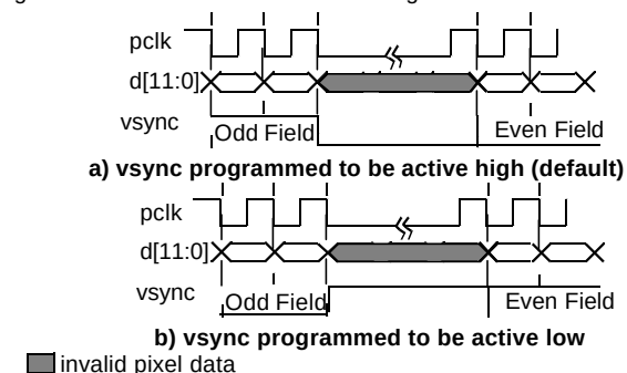
Figure 41. vsync in odd/even Mode
