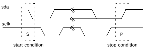
Figure 27. Start/Stop Conditions
