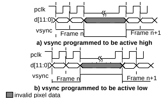
Figure 39. vsync in Level Mode
