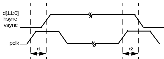
Figure 52. d[11:0] , hsync & vsync to Active High pclk Timing
