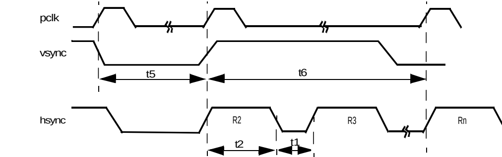
Figure 50. Frame Timing
