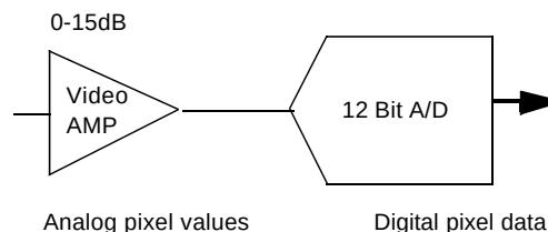
Figure 9: Analog Signals Conditioning & Conversion to Digital
