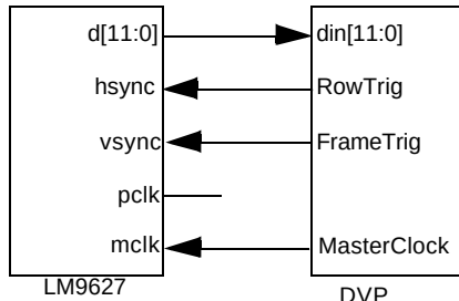
Figure 46. LM9627 in slave mode
