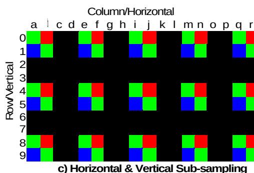
Figure 17: Example 4:2 Sub-sampling
