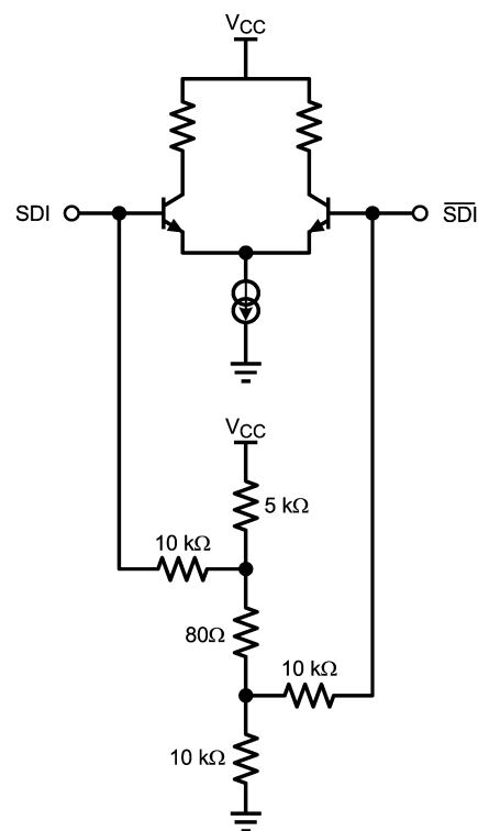
FIGURE 1. Differential Input Stage for SDI and \overline{SDI} .
