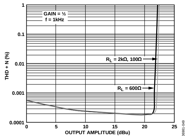
Figure 33. THD + N vs. Output Amplitude, G = \frac{1}{2}
