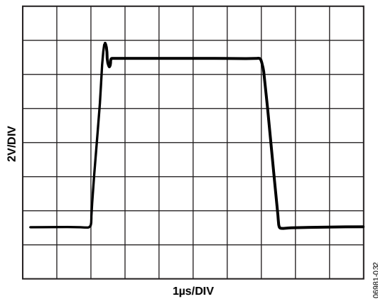
Figure 28. Large Signal Pulse Response, Gain = \frac{1}{2}
