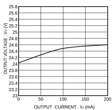
Fig.13 Load regulation
