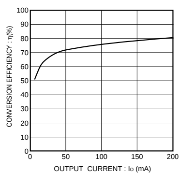
Fig.15 Conversion efficiency
