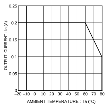
Fig.12 Derating curve
