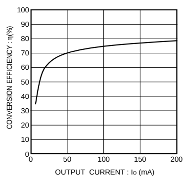
Fig.11 Conversion efficiency
