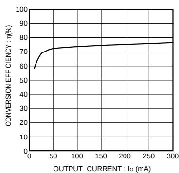
Fig.7 Conversion efficiency
