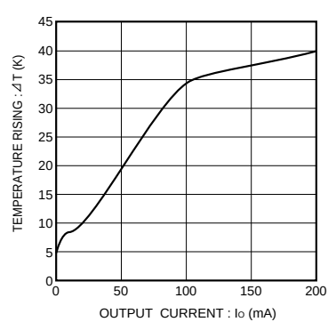
Fig.14 Surface temperature rise
