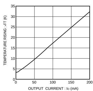
Fig.10 Surface temperature rise
