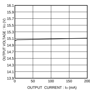
Fig.9 Load regulation
