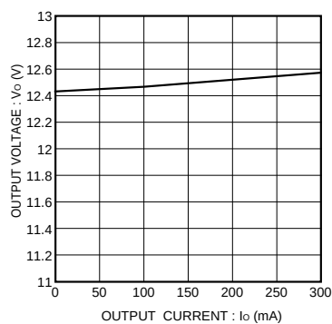
Fig.5 Load regulation
