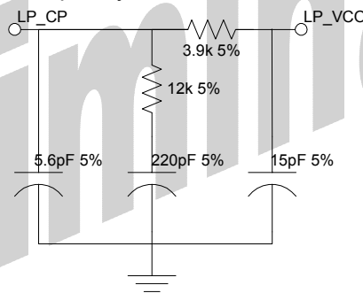
Figure 8.3 - PLL-Loop filter
