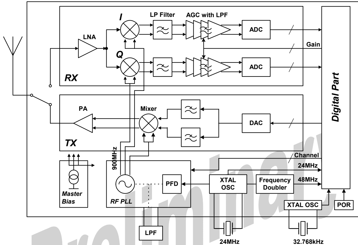
Figure 8.1 - Integrated Analog PHY Layer block diagram
