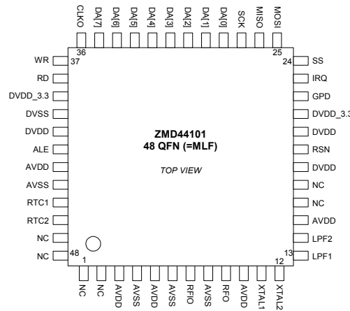
Figure 1.1 - Pin Layout
