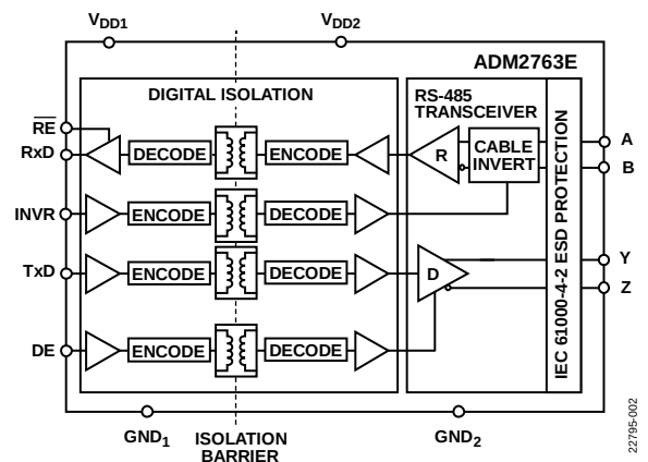
Figure 2. ADM2763E
