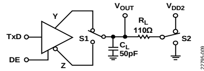
Figure 33. Driver Enable or Disable Time Measurement
