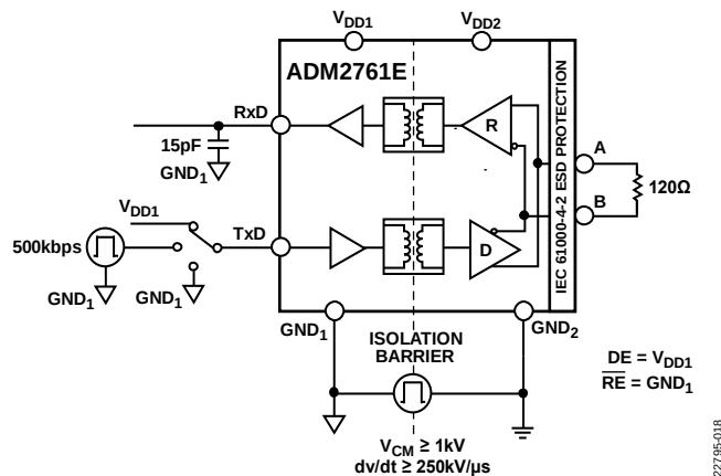
Figure 36. CMTI Test Diagram, Half-Duplex
