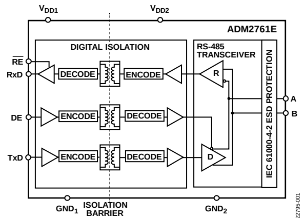
Figure 1. ADM2761E
