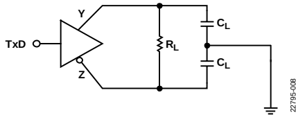
Figure 32. Driver Propagation Delay Measurement
