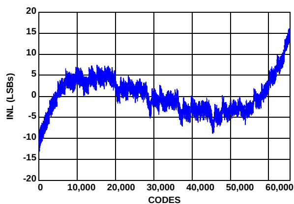
FIGURE 10. INTEGRAL NONLINEARITY
