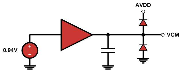
FIGURE 48. VCM_OUT OUTPUT
