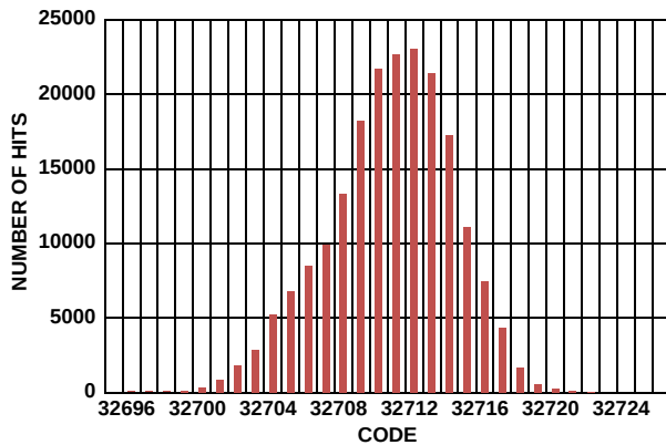
FIGURE 12. NOISE HISTOGRAM
