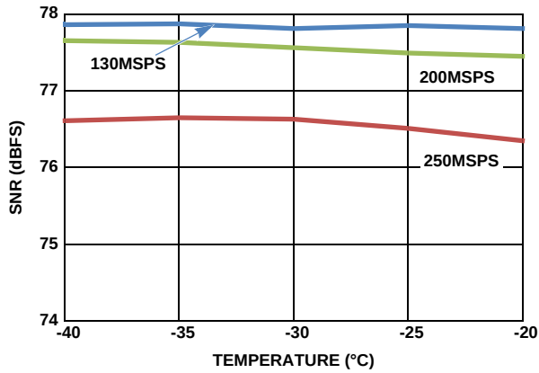
FIGURE 20. TYPICAL SNR PERFORMANCE vs TEMPERATURE, DEVICE CALIBRATED AT -40^{\circ}\text{C} , f_{\text{IN}} = 105\text{MHz} , -2\text{dBFS}
