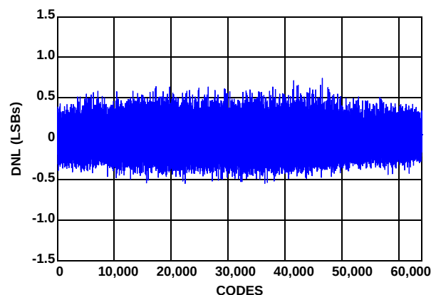
FIGURE 9. DIFFERENTIAL NONLINEARITY
