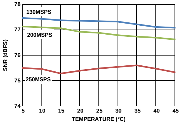
FIGURE 22. TYPICAL SNR PERFORMANCE vs TEMPERATURE, DEVICE CALIBRATED AT +25^{\circ}\text{C} , f_{\text{IN}} = 105\text{MHz} , -2\text{dBFS}
