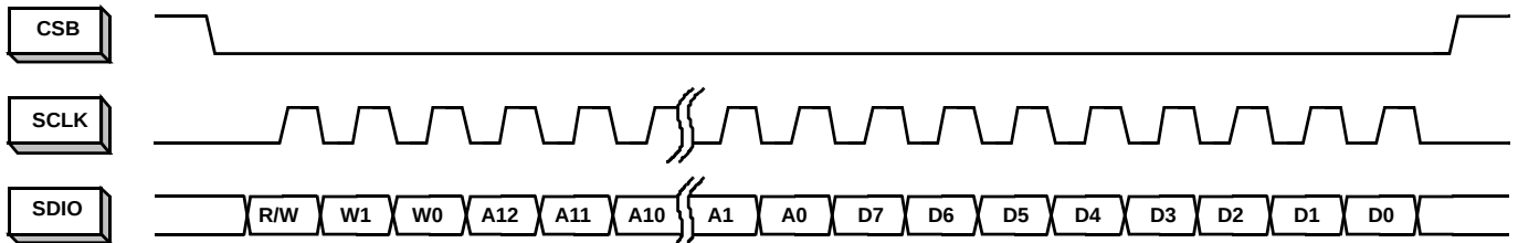
FIGURE 35. MSB-FIRST ADDRESSING
