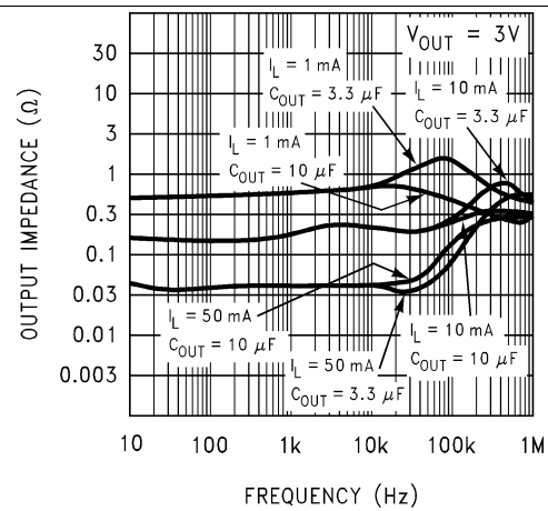
Figure 26. Output Impedance vs Frequency
