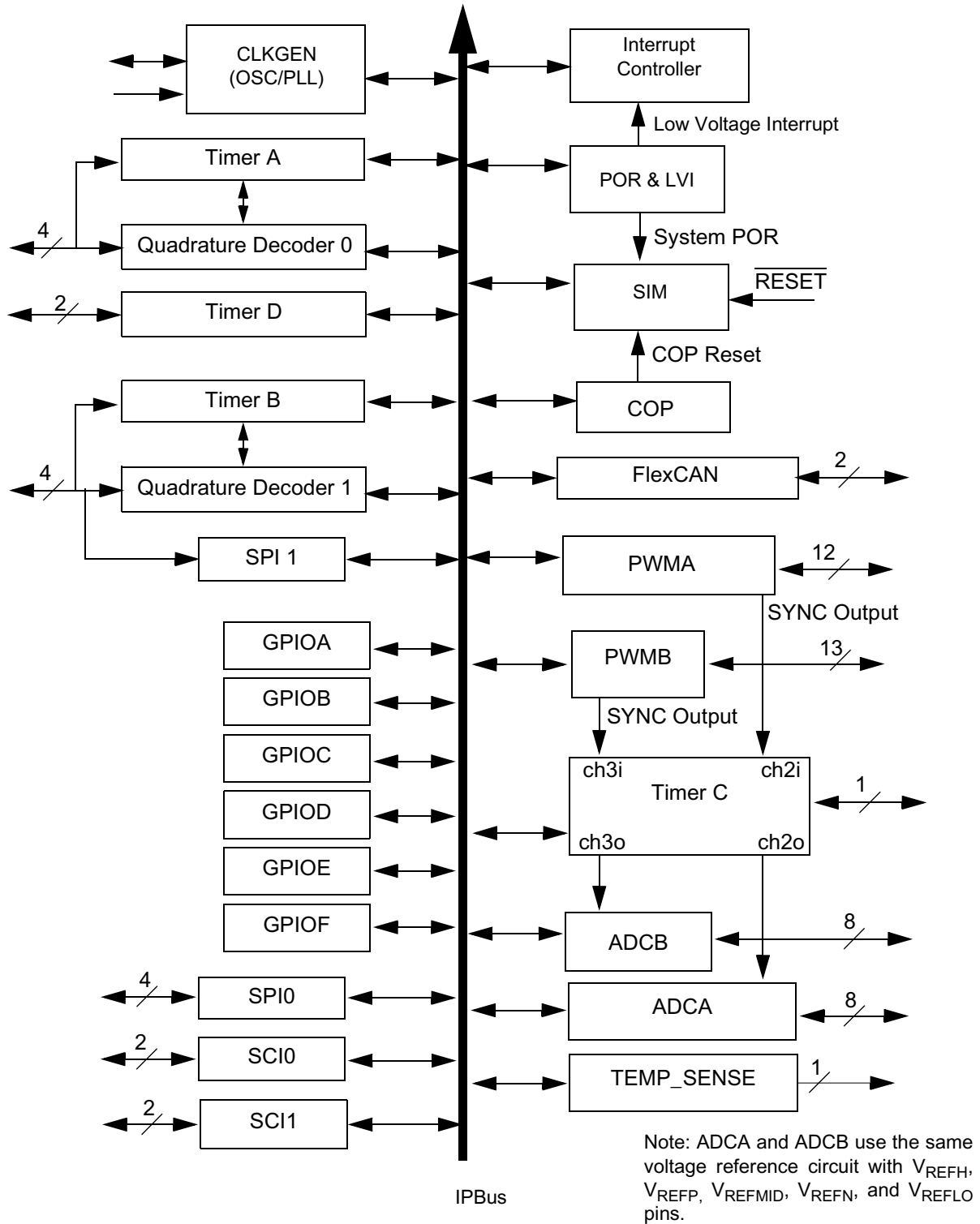
Figure 1-2 Peripheral Subsystem
