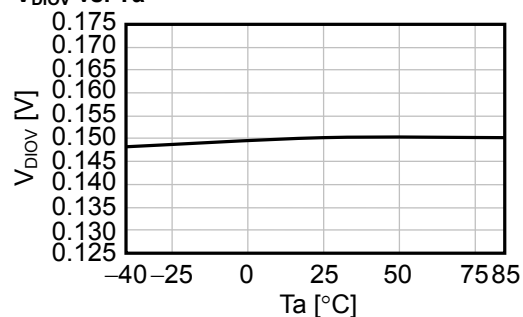
2.7 V_{DIOV} vs. T_a
