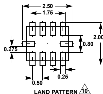
LAND PATTERN \triangle 10
