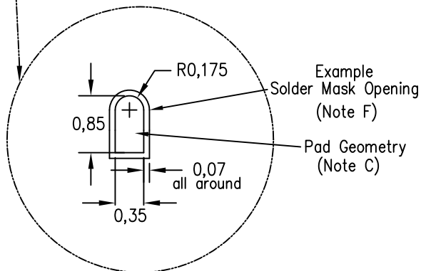
Example Non Solder Mask Defined Pad
