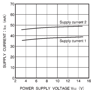
Fig.11 Supply current vs. power supply voltage (BA6417F)
