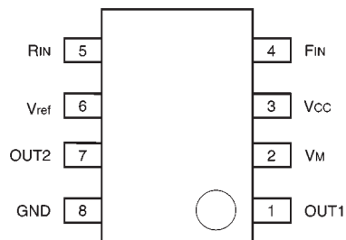
Fig.1 Pin assignments
