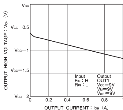
Fig.12 Output high level voltage vs. output current
