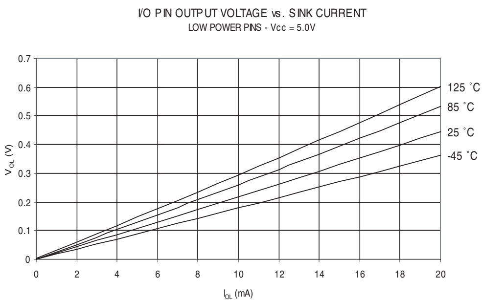
Figure 30-20. I/O pin Output Voltage vs. Sink Current ( V_{CC} = 5V )
