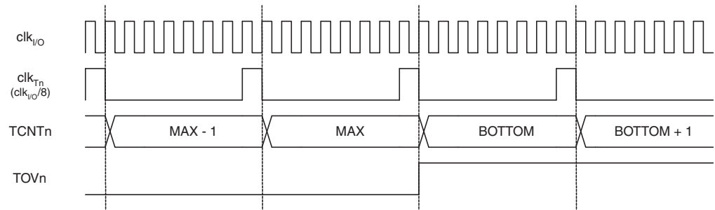
Figure 20-9. Timer/Counter Timing Diagram, with Prescaler ( f_{clk\_I/O}/8 )
