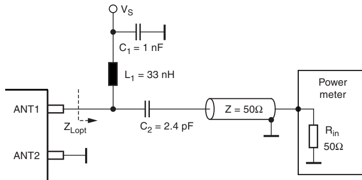
Figure 8-4. Output Power Measurement ATA8742
