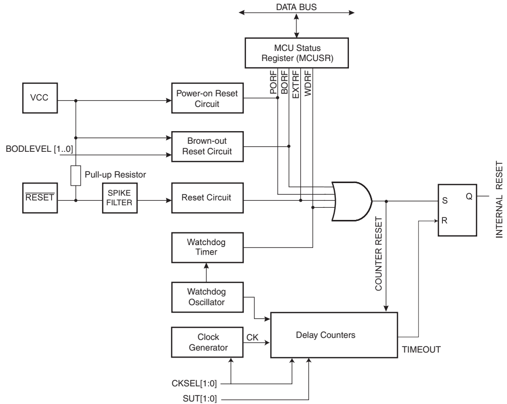
Figure 16-1. Reset Logic
