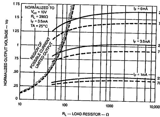
H11V OUTPUT VOLTAGE vs. LOAD RESISTOR
