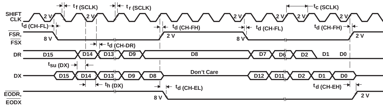
Figure 4-4. Byte-Mode Timing
