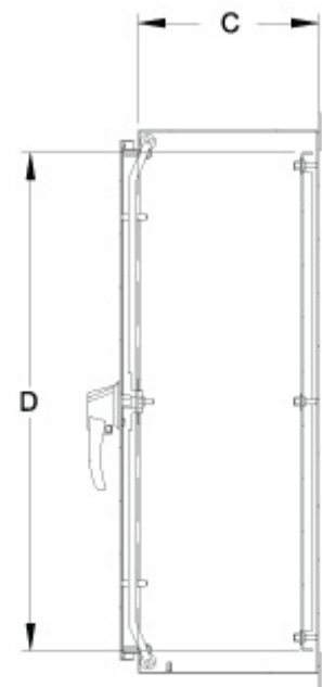
Section Y-Y
