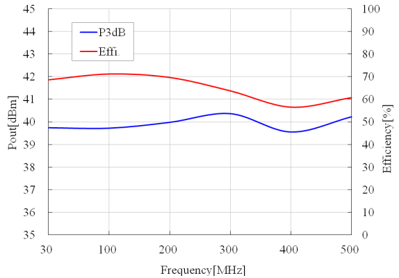
Efficiency vs. Frequency (@P3dB)
