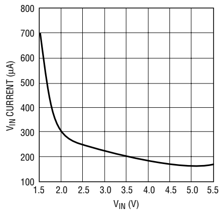
No Load V IN Current in Scan Mode
