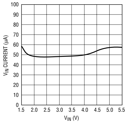
No Load V IN Current in Blank Mode
