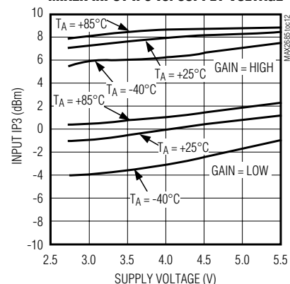
MIXER INPUT IP3 vs. SUPPLY VOLTAGE
