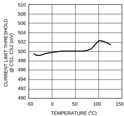
Figure 13. Current Limit Threshold at CS1, CS2 vs Temperature
