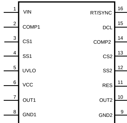
PW Package 16-Pin TSSOP Top View
