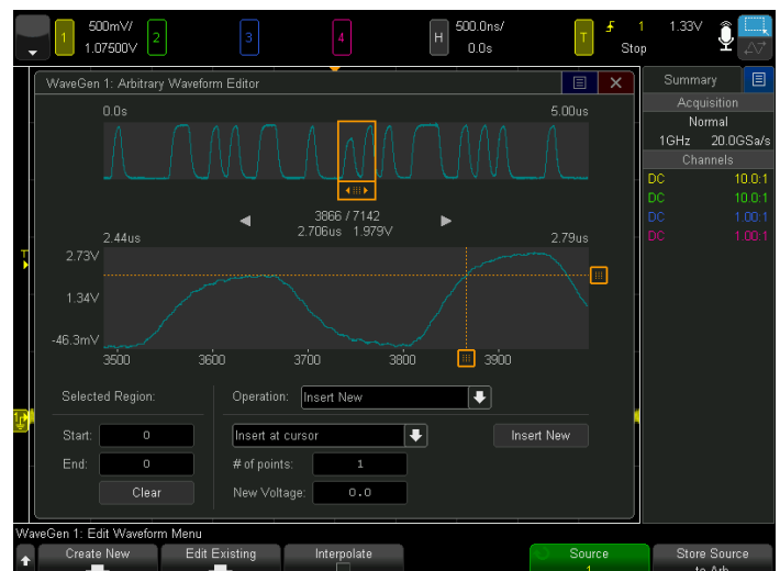
Figure 28. Arbitrary waveform generation signal editing screen.
