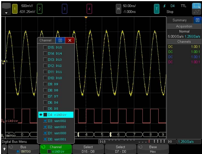
Figure 46. FPGA dynamic probe screen.
