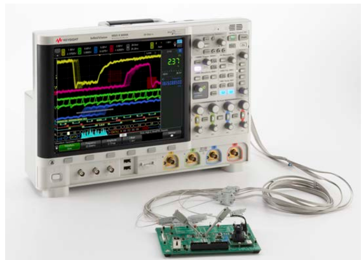
Figure 27. MSO with a new digital channel cable.
