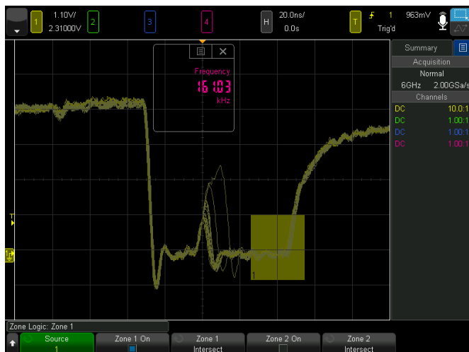
Figure 12. Hardware InfiniiScan Zone triggers immediately.
