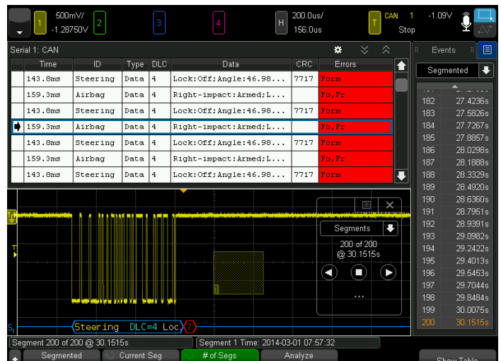
Figure 25. Segmented memory + serial bus decode + InfiniiScan Zone trigger.
