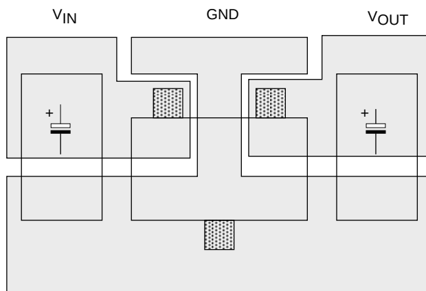
SOT-23-3 BOARD LAYOUT
