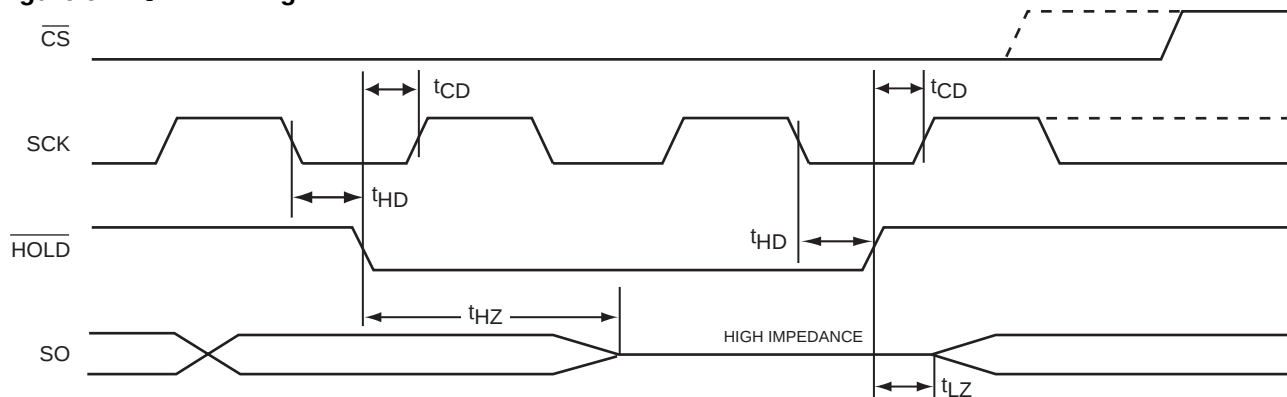
Figure 9. HOLD Timing
