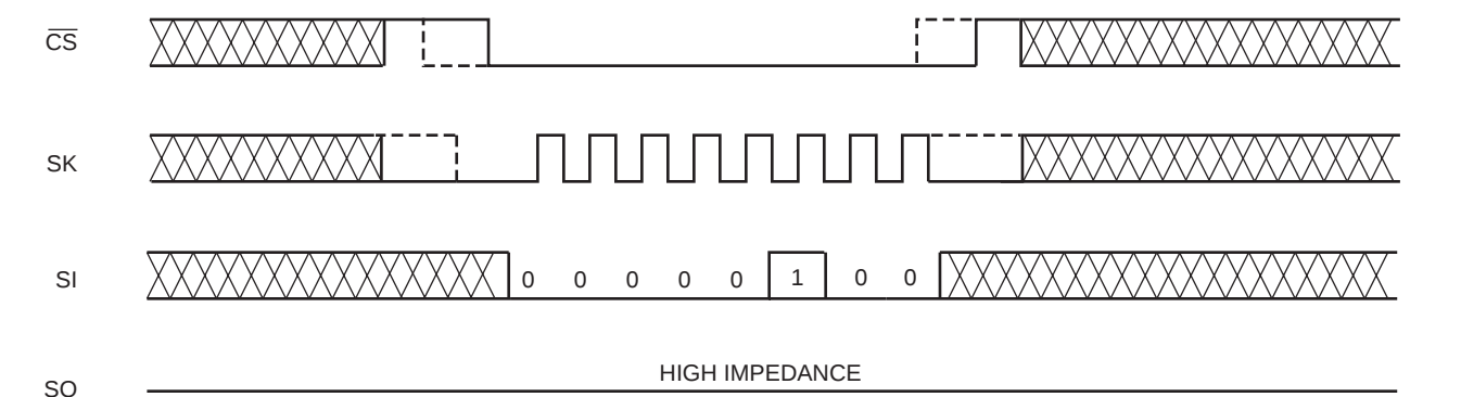
Figure 3. WRDI Instruction Timing
