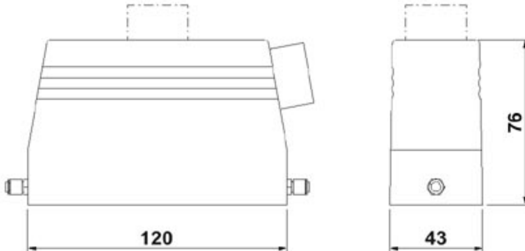
Dimensioned drawing
