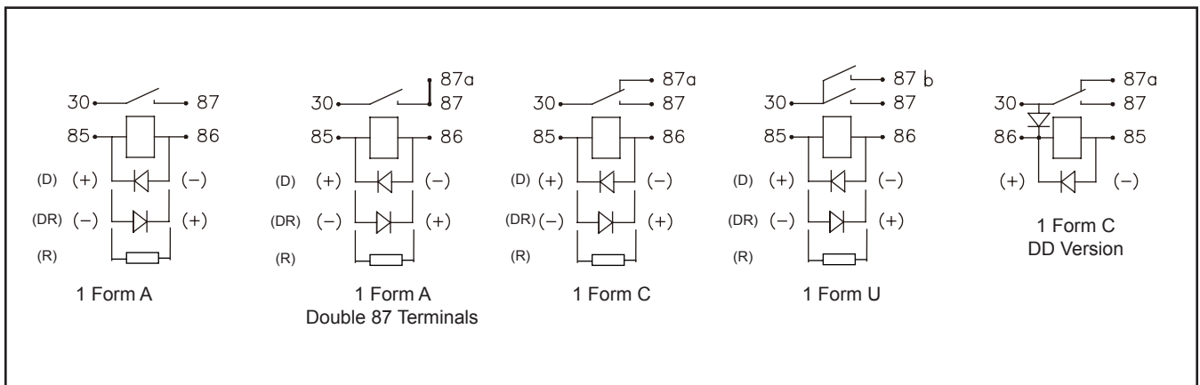
Connection diagrams
