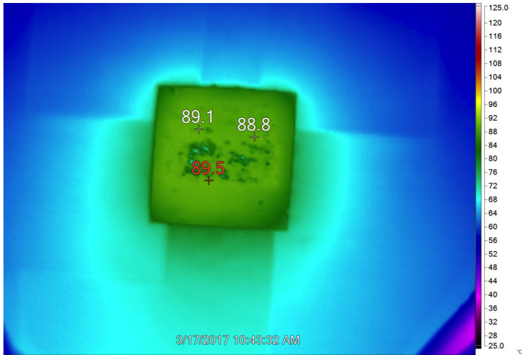
Figure 9. Thermal Performance at V_{IN} = 12V , V_{OUT1} = 1.5V/25A , V_{OUT2} = 3.3V/25A , f_{SW} = 600kHz , T_A = 23^\circ C , No Air Airflow
