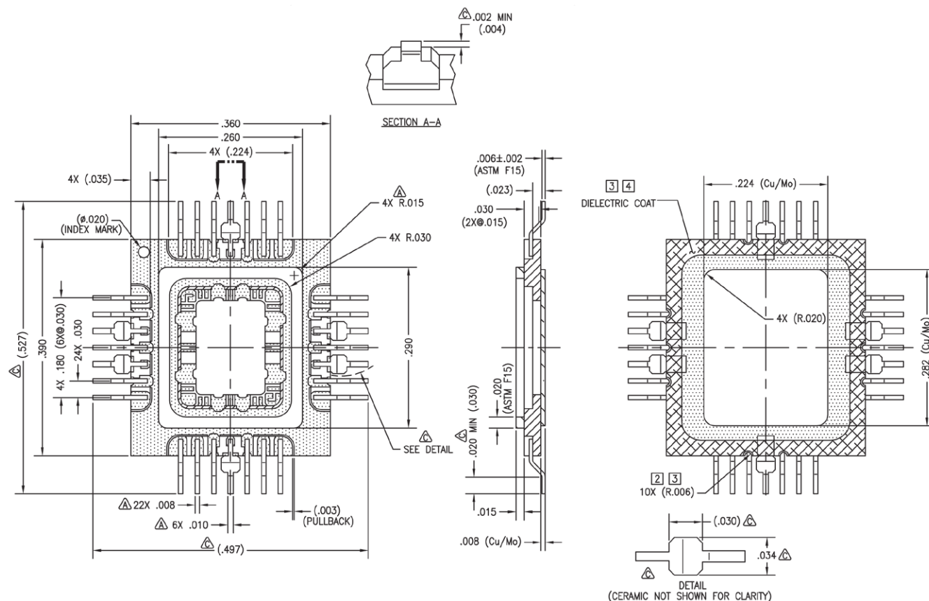
28-lead COFP
