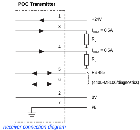
Receiver connection diagram
