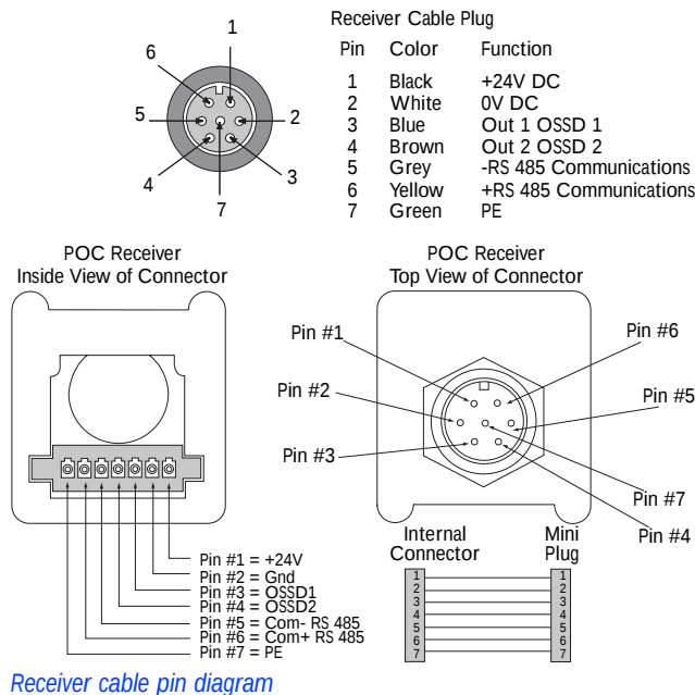
Receiver cable pin diagram
