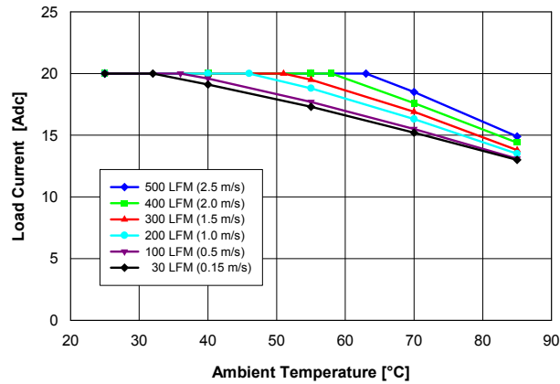
Fig. 2.5V.1: Available load current vs. ambient temperature and airflow rates for V out = 2.5 V converter mounted vertically with V in = 12 V, and maximum MOSFET temperature ≤ 120 °C.
