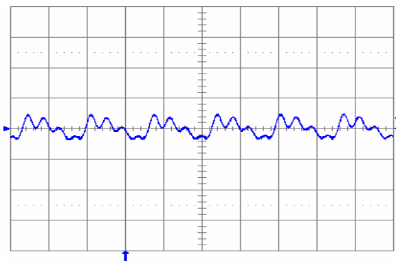
Fig. 1.8V.5: Output voltage ripple (20 mV/div.) at full rated load current into a resistive load with external capacitance 100 \mu F ceramic + 1 \mu F ceramic and V_{in} = 12 V for V_{out} = 1.8 V. Time scale: 2 \mu s/div.
