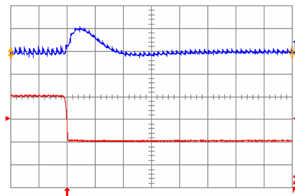
Fig. 1.8V.7: Output voltage response for V_{out} = 1.8 V to negative load current step change from 20 A to 10 A with slew rate of -5 A/ \mu s at V_{in} = 12 V. Top trace: output voltage (200 mV/div.); Bottom trace: load current (5 A/div.). C_o = 100 \mu F ceramic. Time scale: 20 \mu s/div.
