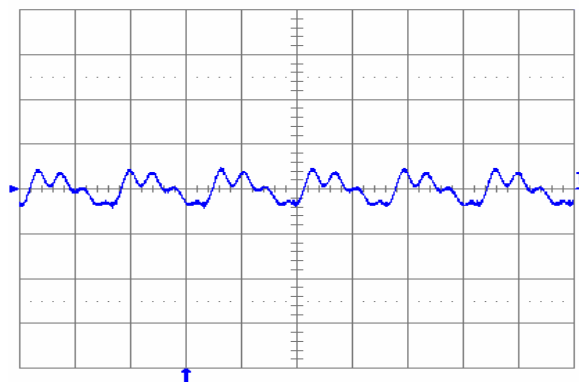
Fig. 2.0V.5: Output voltage ripple (20mV/div.) at full rated load current into a resistive load with external capacitance 100 \mu F ceramic + 1 \mu F ceramic and V_{in} = 12 V for V_{out} = 2.0 V. Time scale: 2 \mu s/div.
