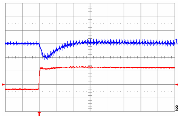
Fig. 2.0V.6: Output voltage response for V_{out} = 2.0 V to positive load current step change from 10 A to 20 A with slew rate of 5 A/ \mu s at V_{in} = 12 V. Top trace: output voltage (200 mV/div.); Bottom trace: load current (5 A/div.). C_o = 100 \mu F ceramic. Time scale: 20 \mu s/div.
