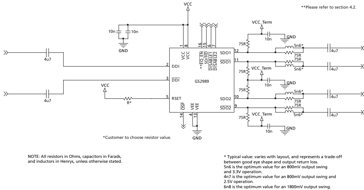
Figure 5-1: Typical Application Circuit
