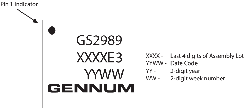
Figure 6-4: Marking Diagram
