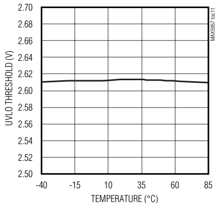
3.3VAUXON UNDERVOLTAGE LOCKOUT THRESHOLD vs. TEMPERATURE
