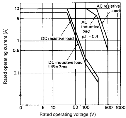
Maximum switching capacity MK2P-S, MK3P5-S
