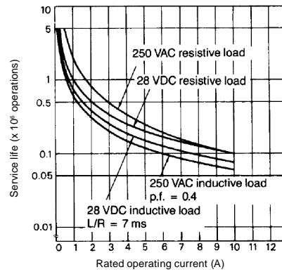
Electrical service life MK2P-S, MK3P5-S
