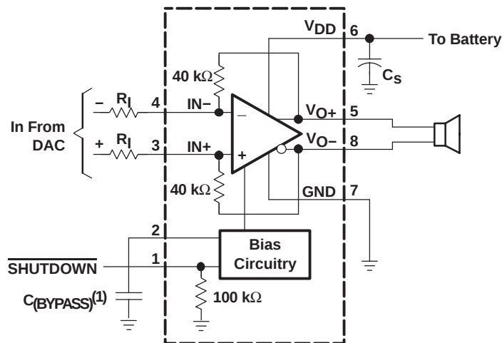
Figure 15. Typical Differential Input Application Schematic
