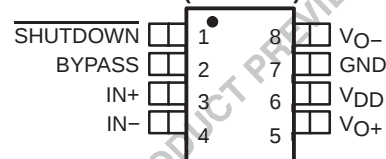
DGN Package (TOP VIEW)
