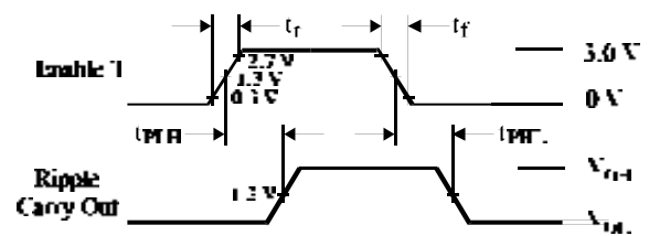
Figure 2. Switching Waveform
