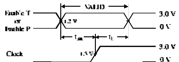
Figure 4. Switching Waveform
