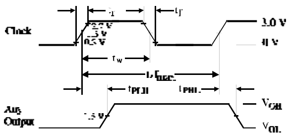
Figure 1. Switching Waveform
