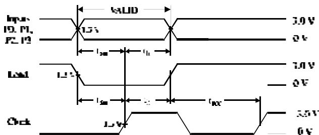
Figure 3. Switching Waveform
