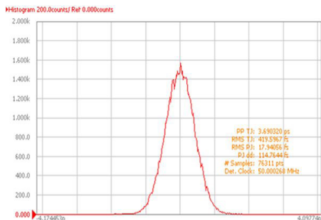
Frequency - 50.000MHz
