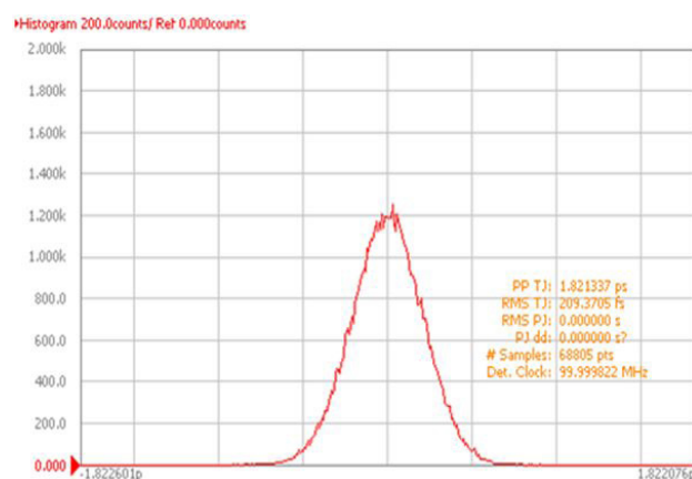
Frequency - 100.000MHz
