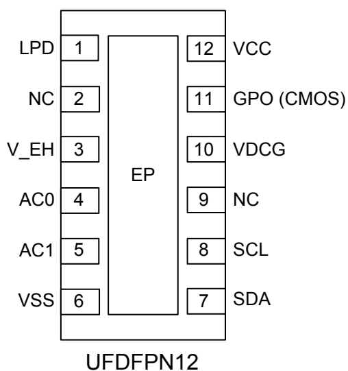
Figure 6. ST25DVxxKC 12-pin UDFPN12 package connections
