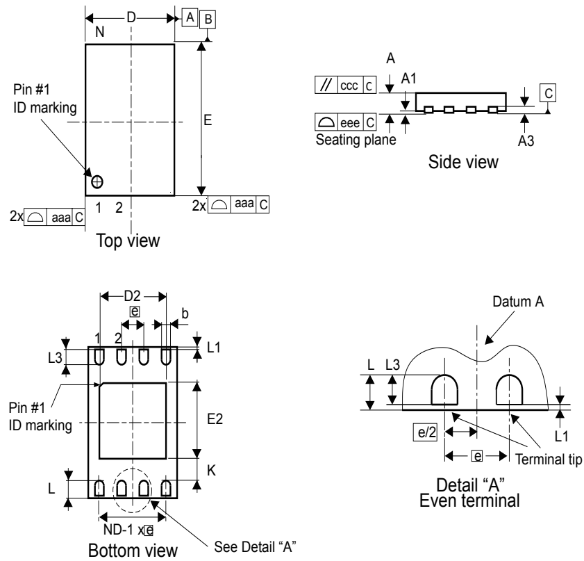
Figure 88. UFDFN8 - Outline
