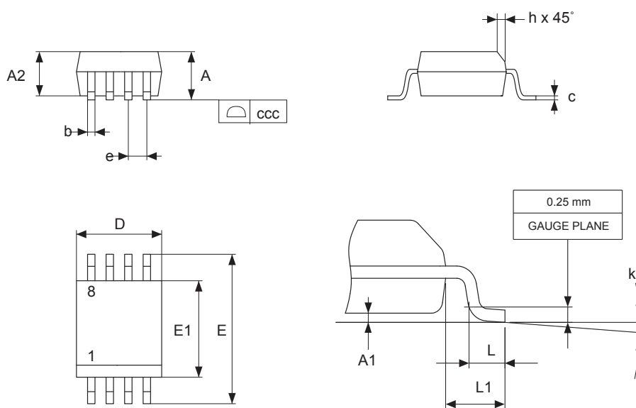
Figure 84. SO8N – Outline
