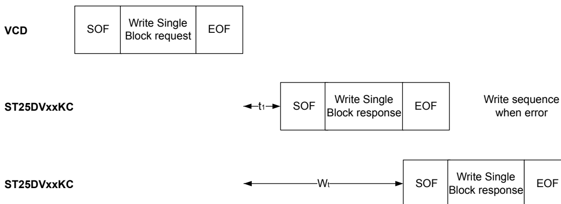
Figure 43. Write Single Block frame exchange between VCD and ST25DVxxKC
