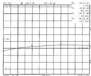
KEK-706H (COUPLING)
