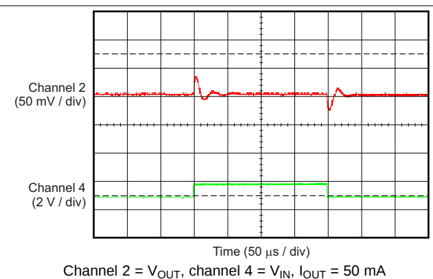
Figure 36. TPS70912-Q1 Line Transient (2.7 V to 3.7 V)
