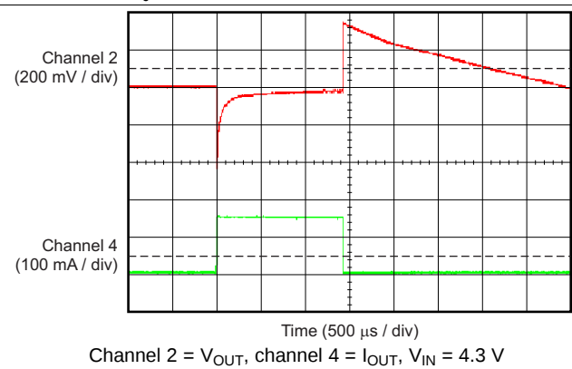
Figure 32. TPS70933-Q1 Load Transient (1 mA to 150 mA)
