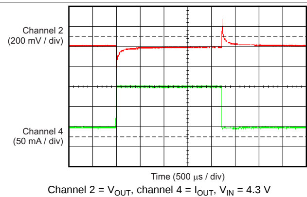
Figure 34. TPS70933-Q1 Load Transient (50 mA to 150 mA)
