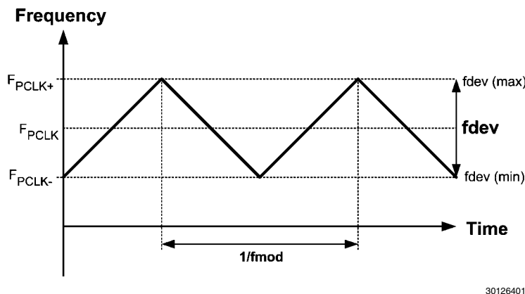
FIGURE 1. SSC Triangle Modulation
