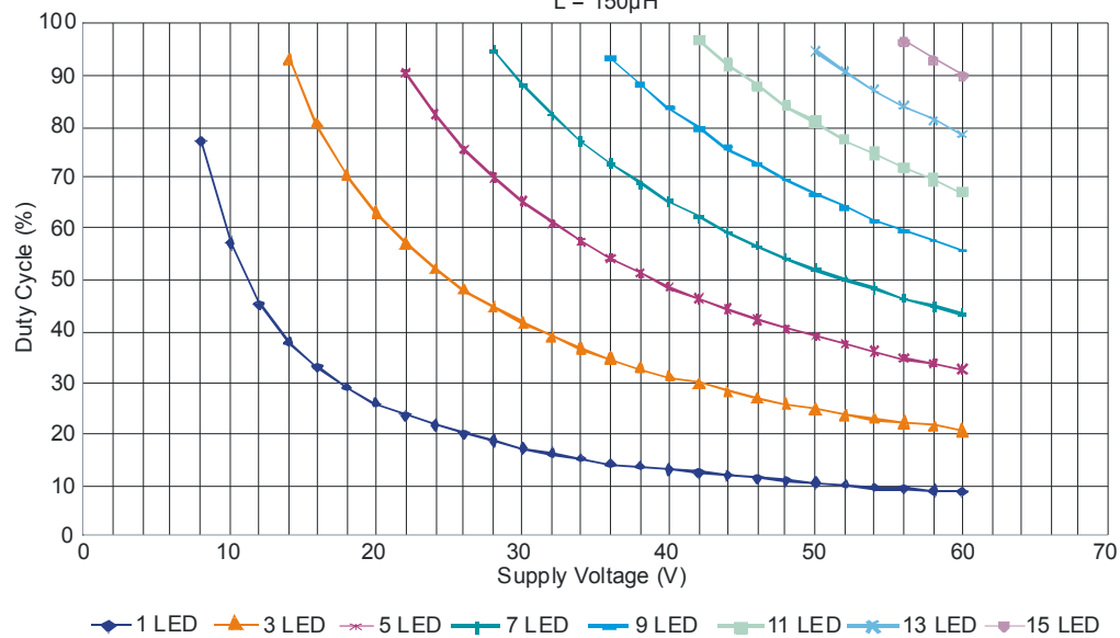
ZXLD1362 Duty Cycle L = 150 \mu H
