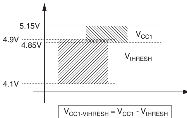
Figure 5-2. Correlation between VCC Output Voltage and Reset Threshold
