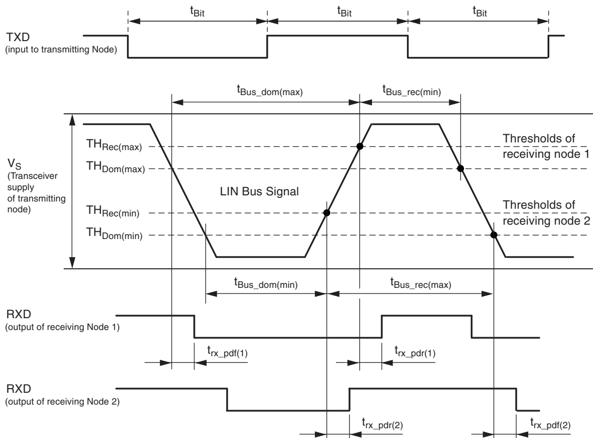
Figure 5-5. Definition of Bus Timing Parameters
