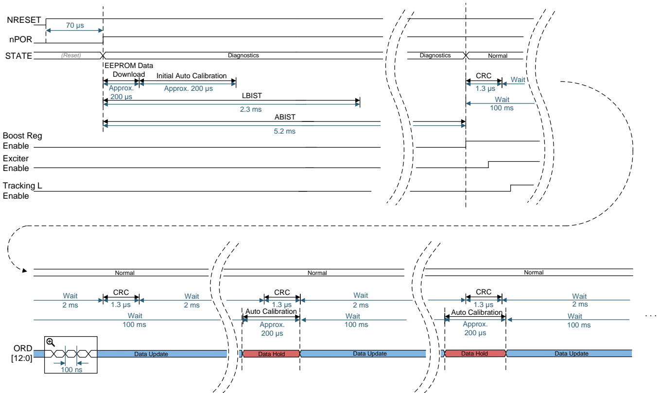
Figure 2. Power-Up Timing Diagram
