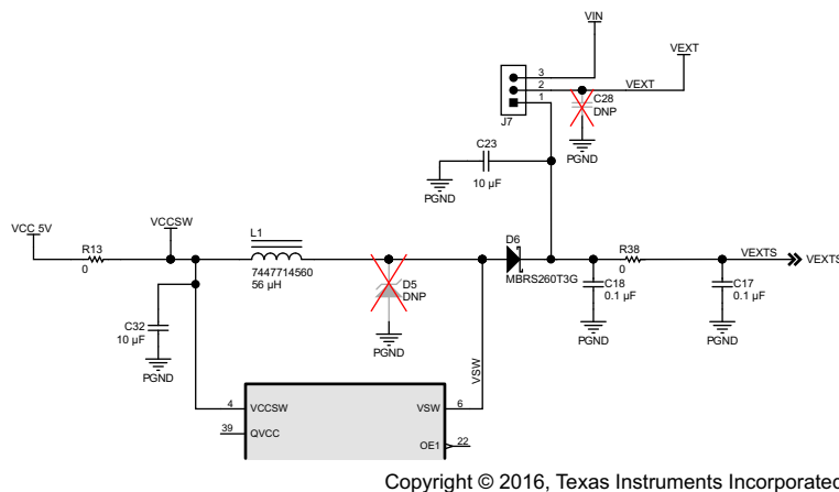
Figure 85. Boost Circuit Schematic
