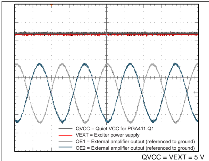
Figure 74. Exciter Amplifier
