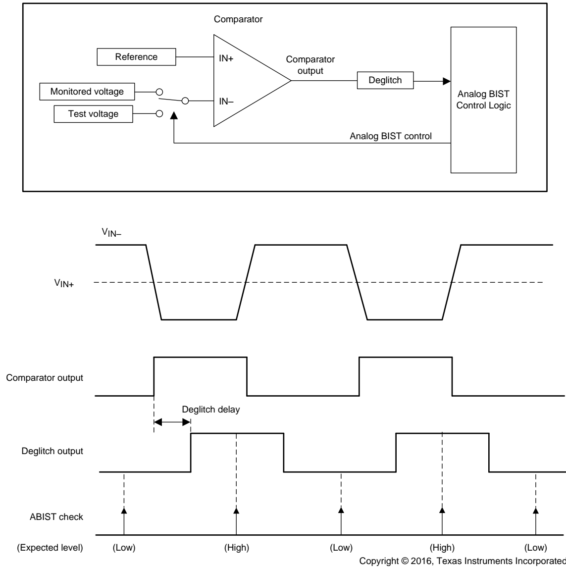
Figure 38. BIST
