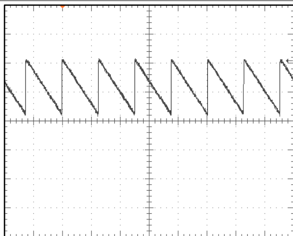
Figure 76. AOUT Signal (With No Resolver Connected)
