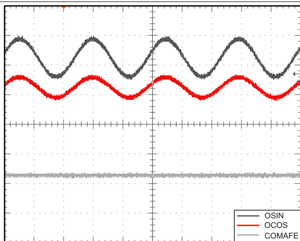
Figure 78. Analog Front-End (AFE) Outputs
