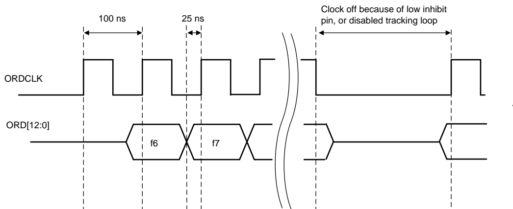
Figure 33. ORD Timing Characteristics
