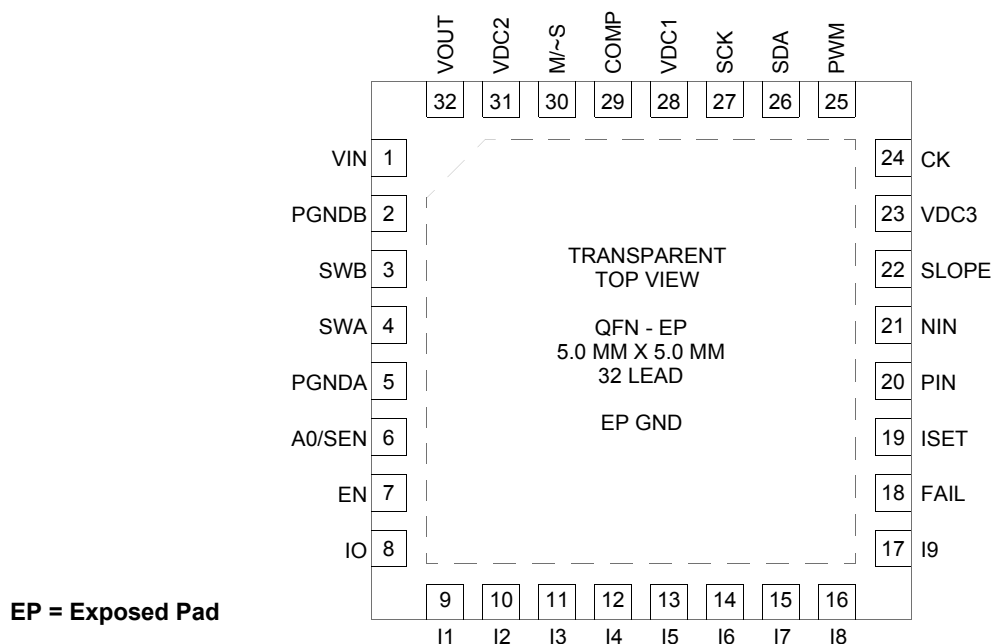
Figure 4. 34844 Pin Connections
